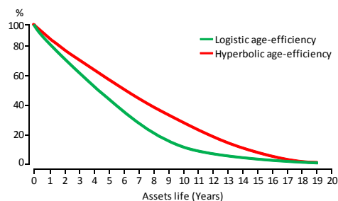
Diagram 3: Age-price functions
